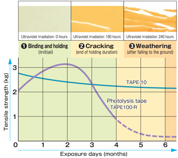
[Decomposition of 100-R tape for grapes (Delaware)] Testing using a sunshine weather meter (condition: temperature 60°C)
