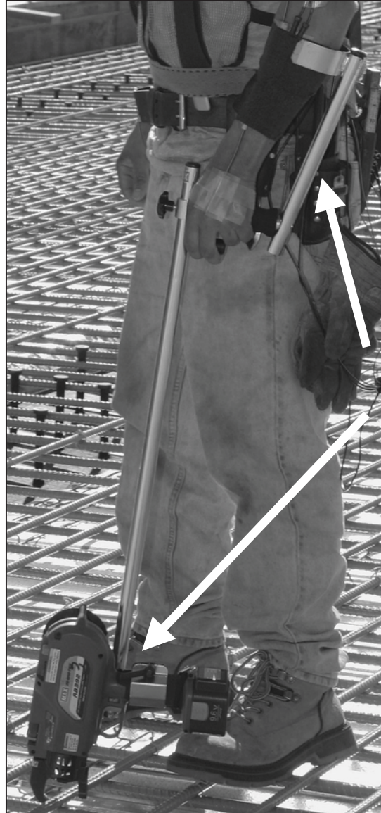
Figure 5 MAX-USA RB-392 Battery powered tier with adjustable extension (BPT+E) (plan to use image from manufacturer)
