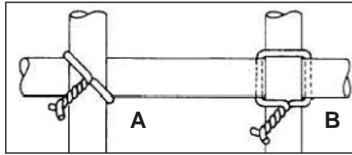
Figure 2 Ties used to secure rebar together
